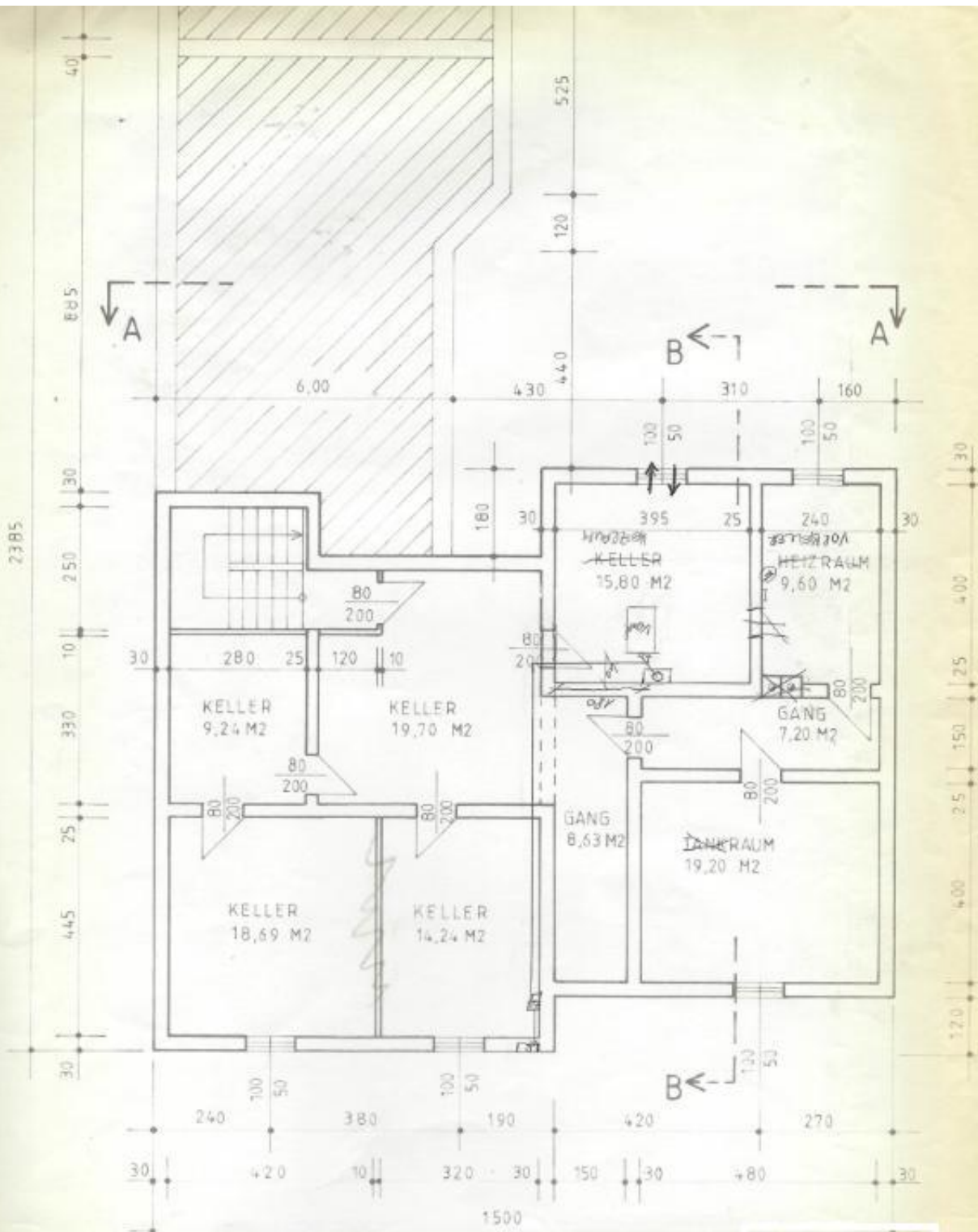
KELLER M = 1:100
