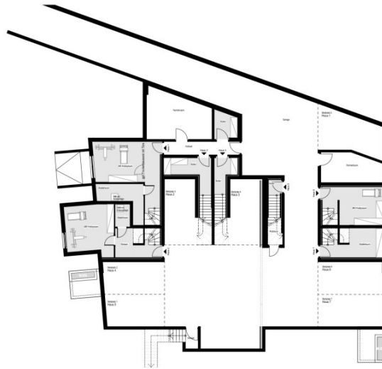
Tiefgarage M = 1:200
