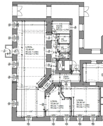
GRUNDRISS SOUTERRAIN M=1:100
