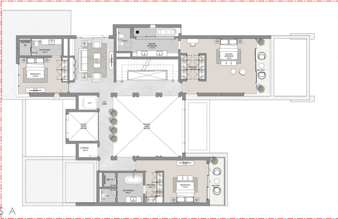
5-Bedroom villa type A- First floor plan
