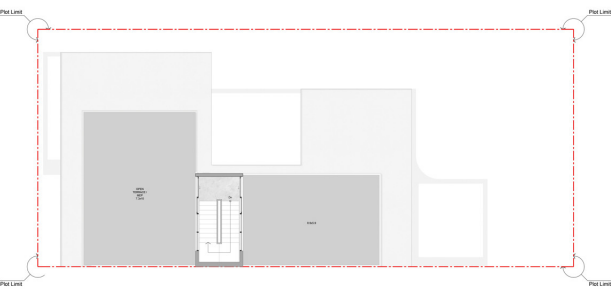
4-Bedroom villa type A- Terrace floor plan
