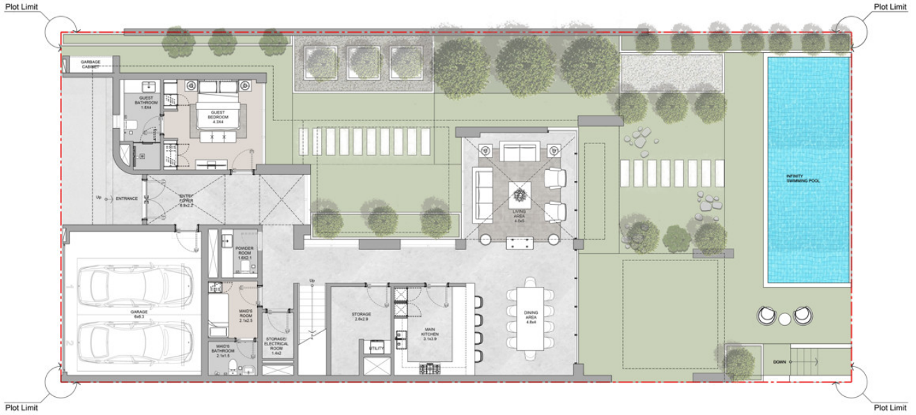
4-Bedroom villa type A- Ground floor plan
