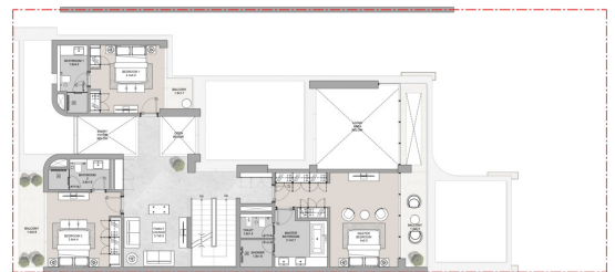
4-Bedroom Villa type A- First floor plan
